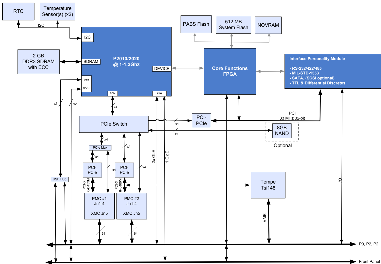
Figure 1: SVME/DMV-194 Core Processing Architecture
